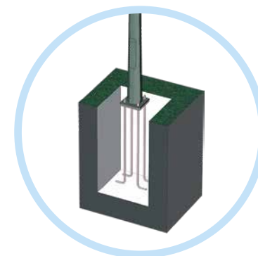
FLANGE CONNECTION
