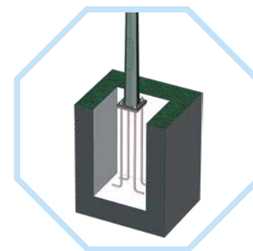
FLANGE CONNECTION
