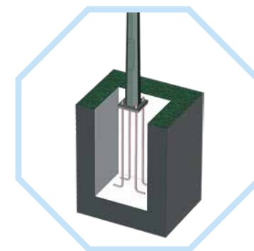
FLANGE CONNECTION
